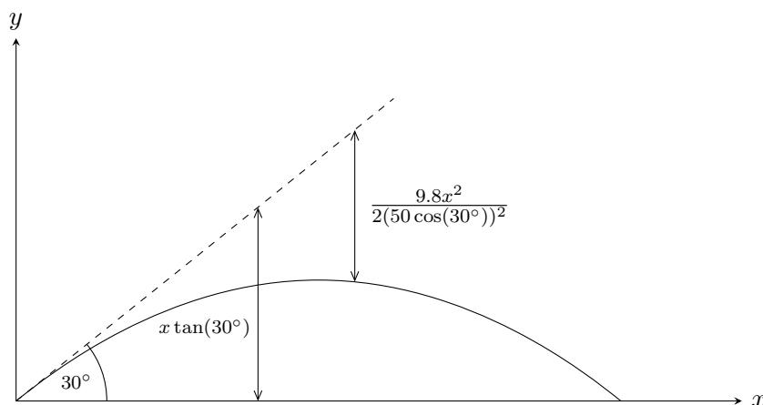
Figure 2.4: Projectile trajectory.
